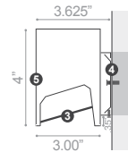
CROSS-SECTION: WW
