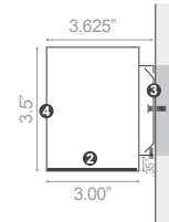
CROSS-SECTION: LAMBERTIAN
