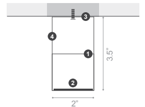
CROSS-SECTION
